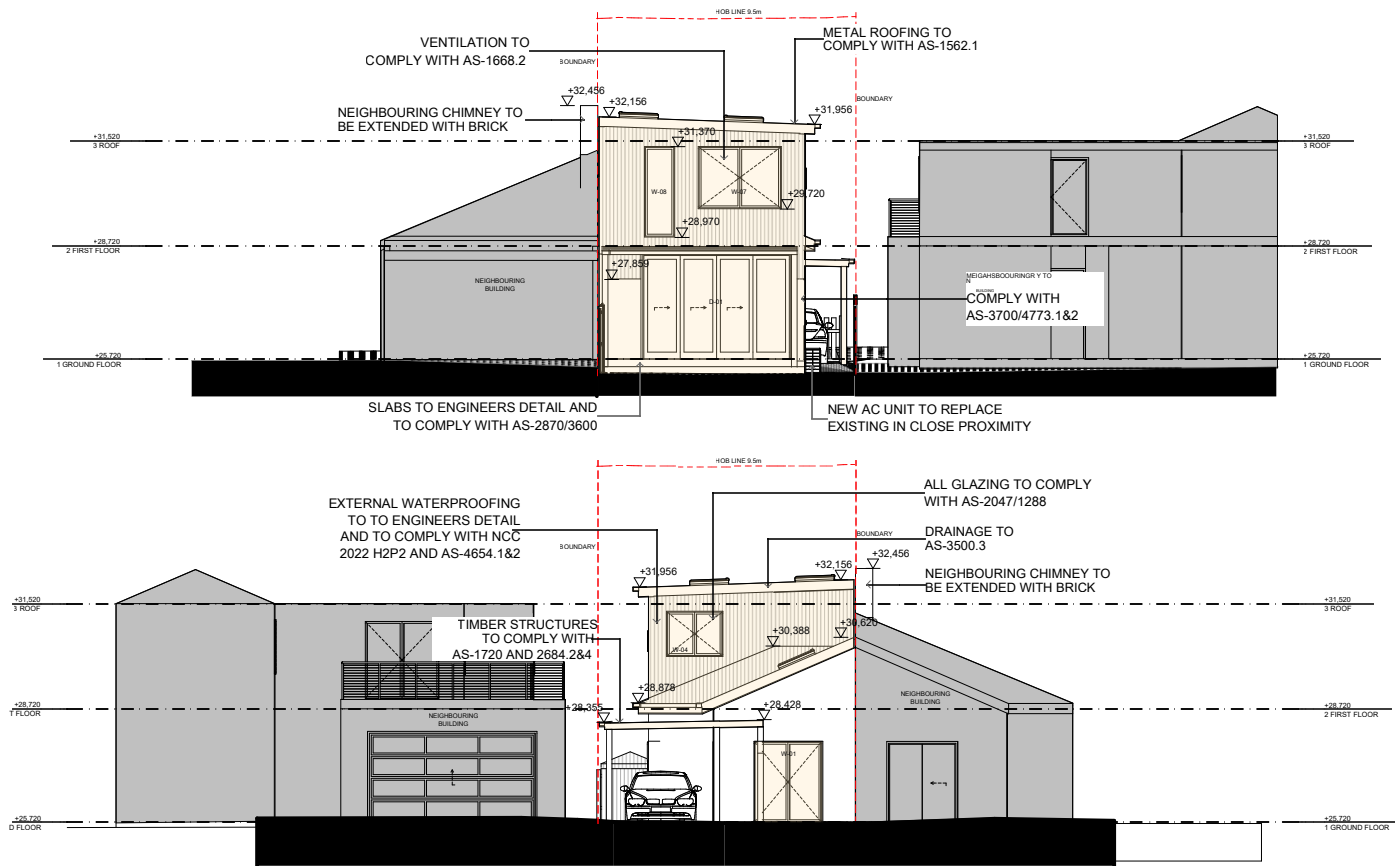
NORTH & SOUTH ELEVATION
